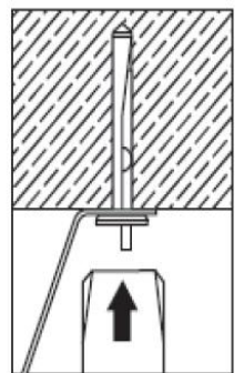
Hammer in anchor.
