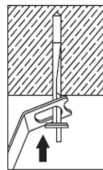
Install anchor with suspended item.
