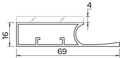
Size: 71 x 13 x 3000 mm
